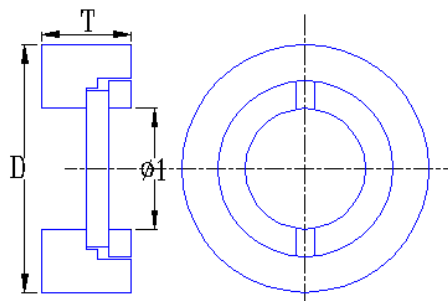
Figure 1: A schematic drawing of a window mount
